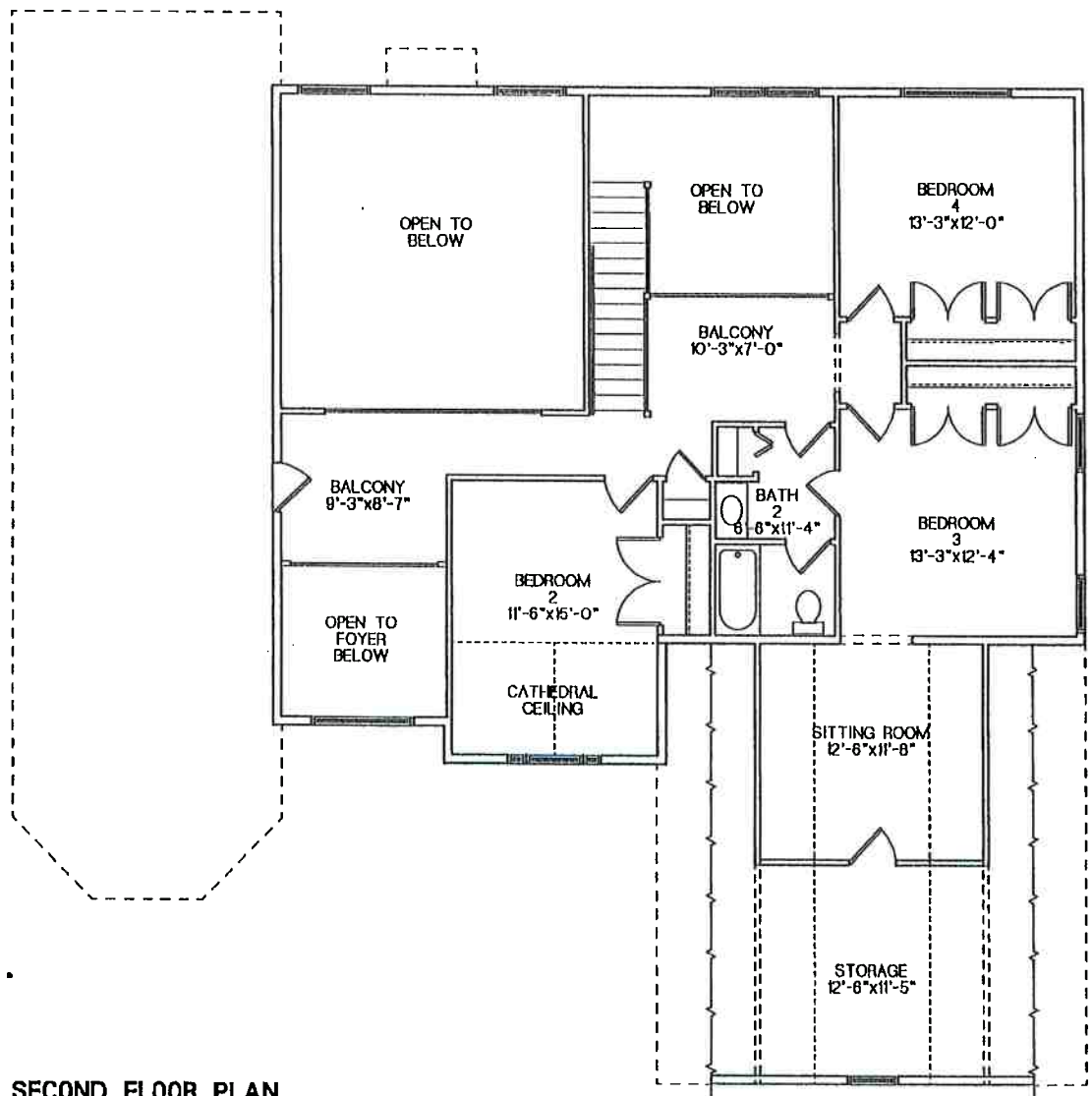
SECOND FLOOR PLAN 1095.08 SQ. FT.
