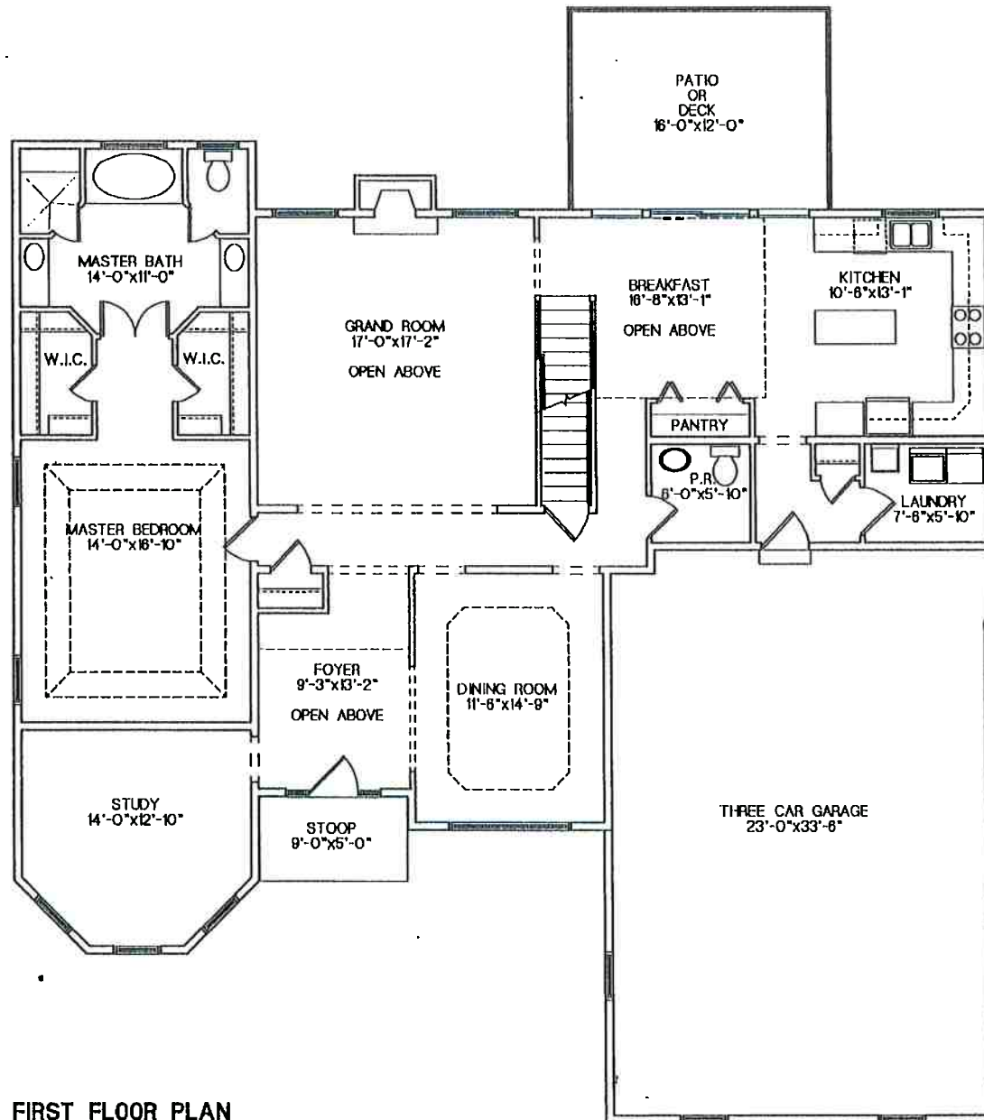
FIRST FLOOR PLAN 60'-0"(W) x 58'-4"(D) 1978.85 SQ. FT.
